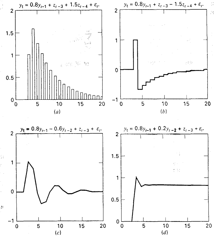
Figure 5.3 Standardized cross-correlograms.
