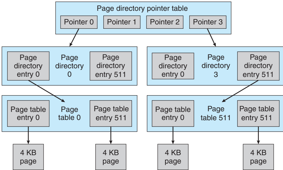
Figure 19.3 Page-table layout.
