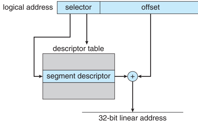
Figure 8.22 IA-32 segmentation.
