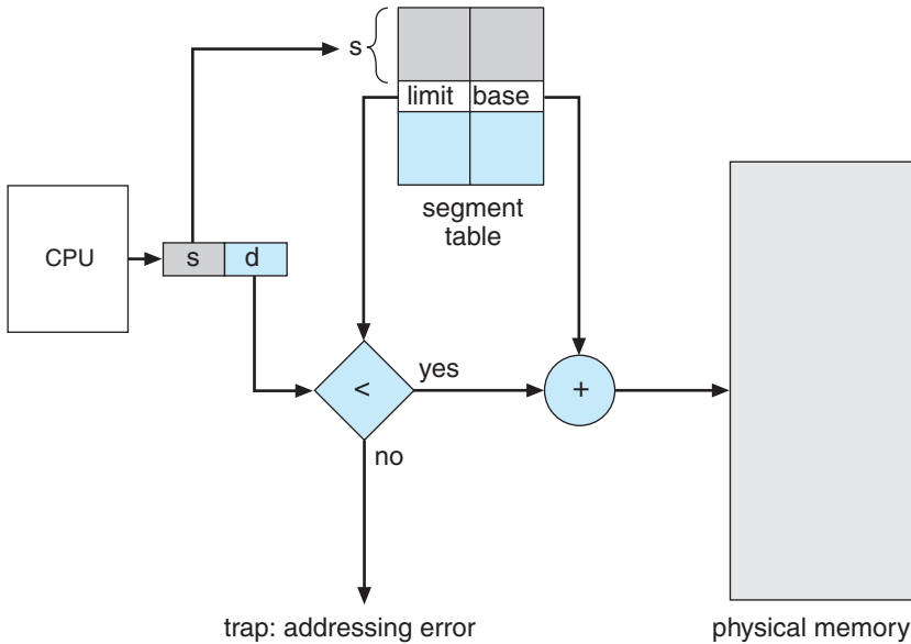
Figure 8.8 Segmentation hardware.
