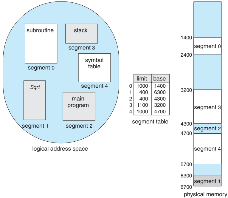
Figure 8.9 Example of segmentation.
