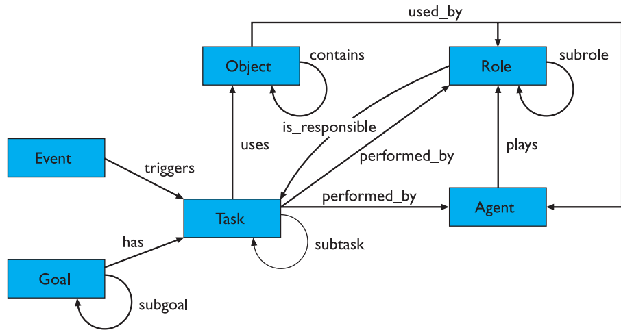
Figure 18.5 GTA ontology
